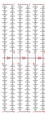
Circuit Diagram
