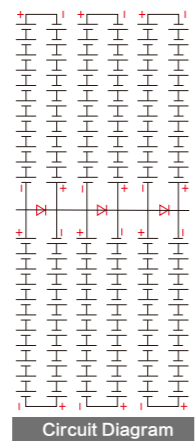
Circuit Diagram
